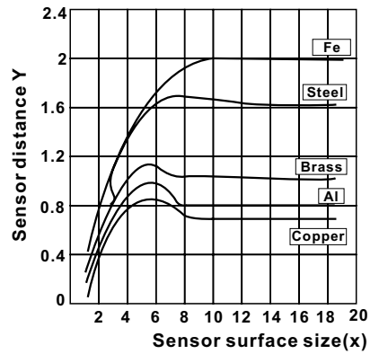
PSH1-M10 Adjusted the sensing distance 2mm with 20mm meta boardl
