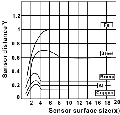
PSH1-D5.4 Adjusted the sensing distance 1mm with 20mm meta boardl
